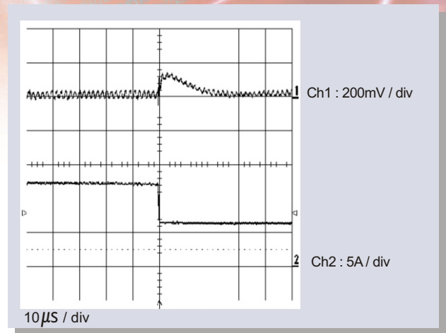
Fig19. Transient Response to Dynamic Load Change from 50% to 100% of full load ( V_{in} = 5.0V , V_o = 3.3V , C_o = 150\mu F \times 2 )
