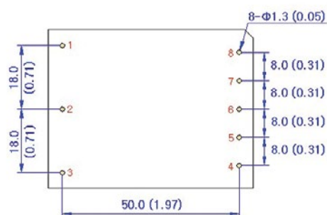
| Mounting Hole (Top View) |
