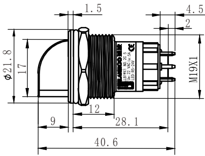
头部防水款 Head waterproofing
