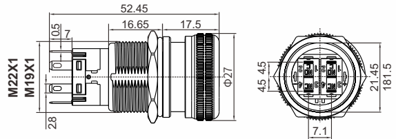
19M5.4 22M5.4急停 19/22M5.4 Stop Button
