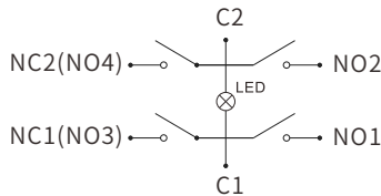
带灯 (3档/6脚) With LED (3rd gear/6-pin)
