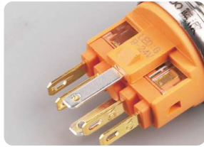
镀金/镀银插脚,导电性好 Silver/Gold Plated Pins
