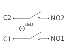
带灯 (2档/4脚) With LED (2rd gear/4-pin)
