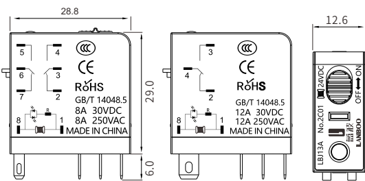
银触点,大电流 Silver contact, High Current
