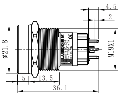
头部防水款 Head waterproofing
