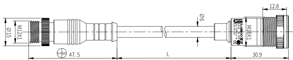
带线全防水款 Fully waterproof with wire
