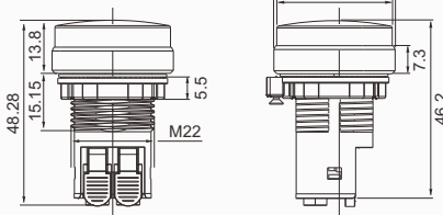
平头指示灯 Flat head indicator light
