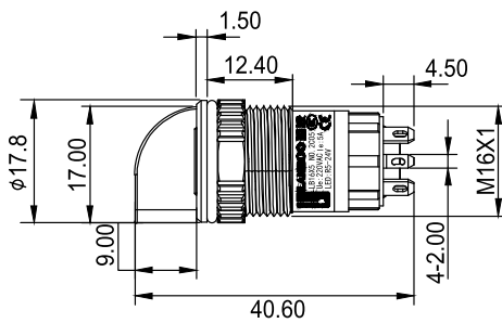
头部防水款 Head waterproofing
