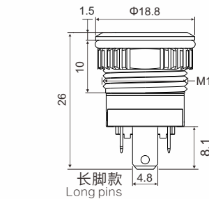
镀银长插脚 Silver Long Plated Pins
