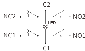
带灯 (2档/6脚) With LED (2rd gear/6-pin)
