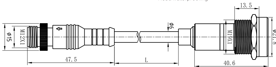
带线全防水款 Fully waterproof with wire
