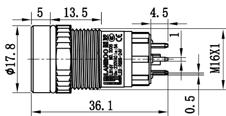
头部防水款 Head waterproofing
