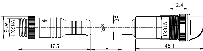
带线全防水款 Fully waterproof with wire
