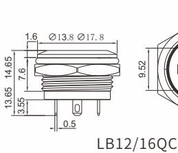
不锈钢外壳 Stainless Steel Shell
