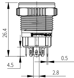
头部防水款 Head waterproofing
