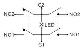
6脚 (2档) 原理图 Schematic diagram of 6-pin (2nd gear)
