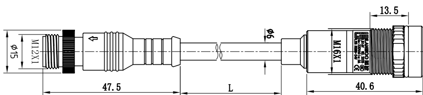
带线全防水款 Fully waterproof with wire
