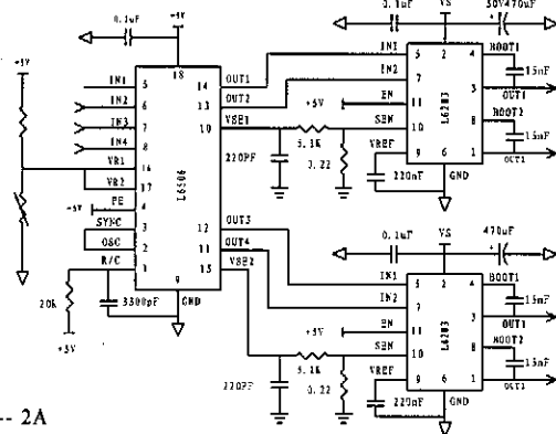
动态性能测试电路 Testing Circuit for Dynamic Performance 4-6, 4-7, 4-8, 4-9.
