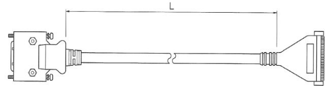
[ CSI02S-□ ]
