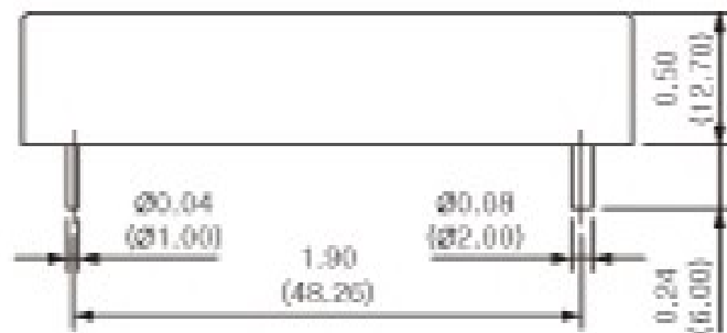
HF-series [ CASE TYPE ]
