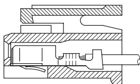
TERMINAL ASSEMBLY DRAWING
