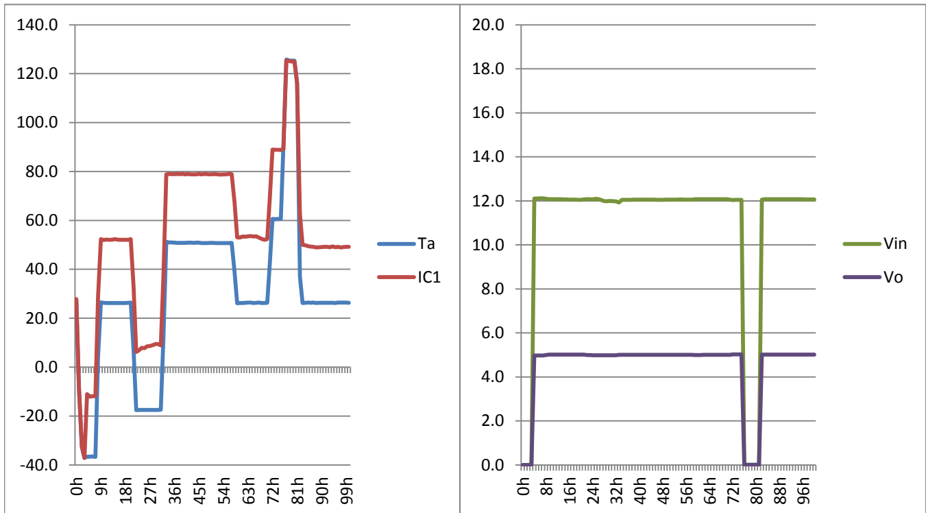
f. Characteristics test results (@ Input Voltage : 12VDC)
