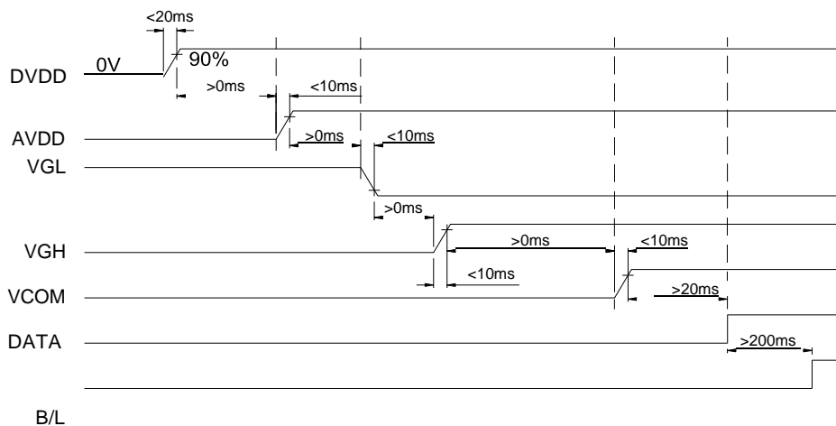
Power on sequence: DVDD → AVDD → VGL → VGH → VCOM → DATA → B/L
