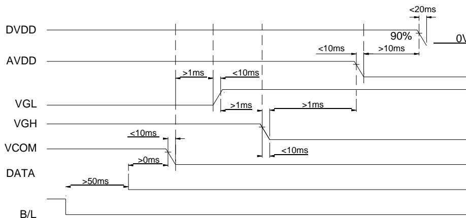
Power off sequence: B/L → DATA → VCOM → VGL → VGH → AVDD → DVDD
