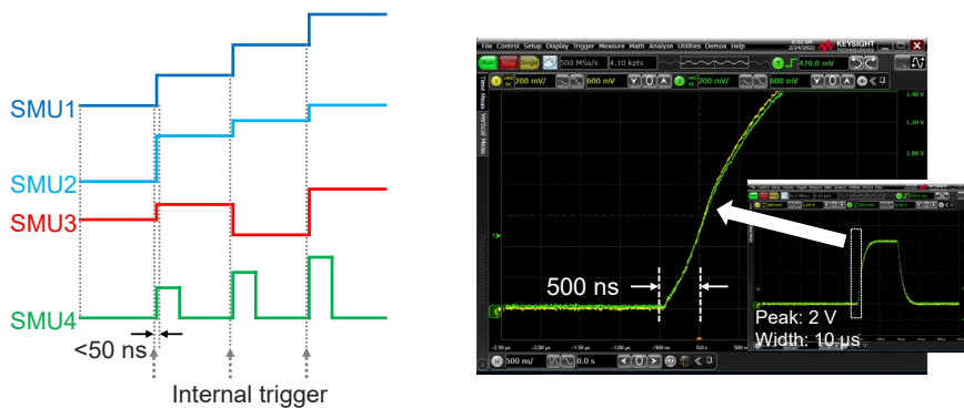
Figure 12. Internal trigger lines enable channel synchronization at less than 50 ns accuracy, and external trigger ports enable synchronization with any piece of external equipment
