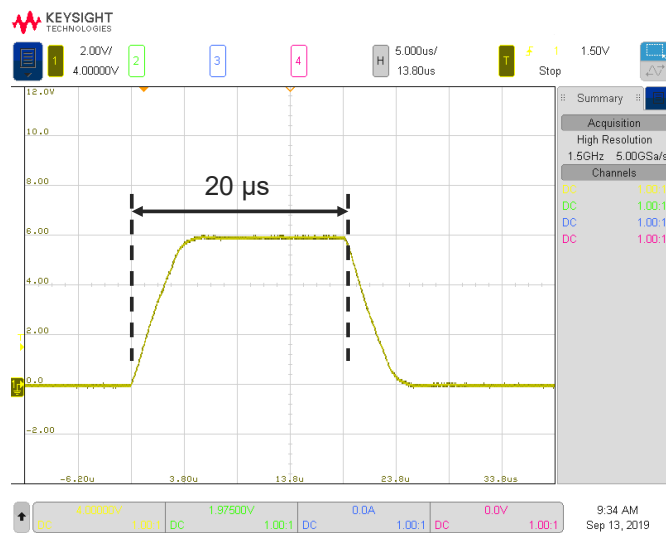
Figure 8. Narrow pulse down to 20 \mu s enables you to suppress the self-heat effect to reveal the true characteristics of the devices
